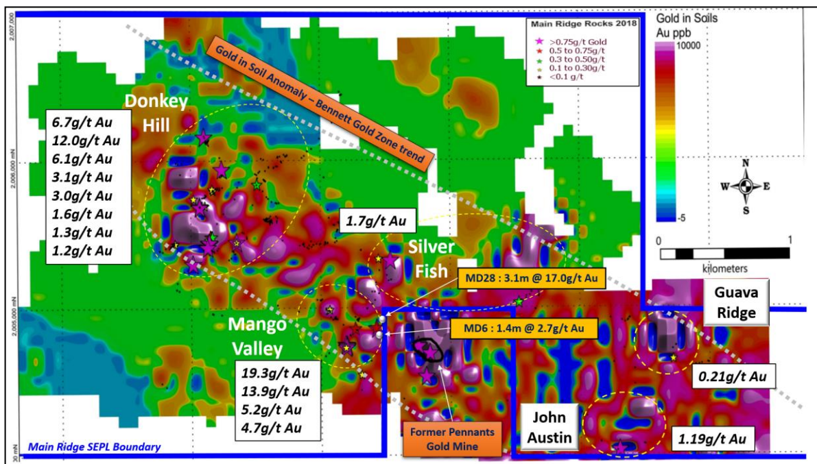
Figure 1: Main Ridge Project area, showing color plot of gold in soil geochemistry (Note - Pennants gold mine does not occur within Carube's Main Ridge SEPL)
