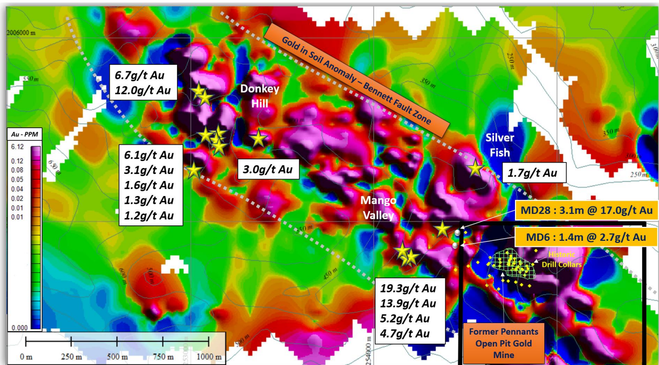
Figure 1: Main Ridge Project area, showing gold in soils and high grade gold in rocks collected at the Donkey Hill, Mango Valley and Silver Fish prospects in respect to the former Pennants Open Pit gold mine. Pennants gold mine does not occur within Carube’s Main Ridge SEPL.
