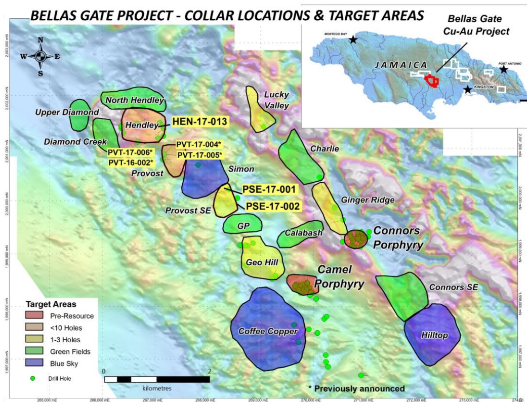
Figure 1: 2017 Drill Locations within the 6.5km by 4.0km copper mineralized belt showing location of HEN-17-013, PSE-17-001 and PSE-17-002
